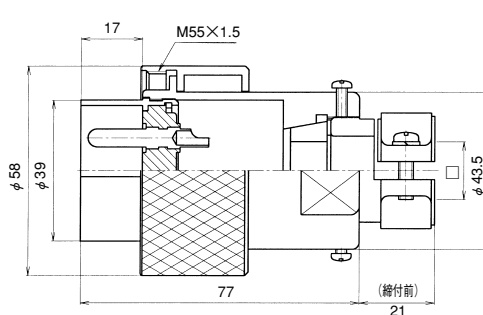
WT-44※-PM□
