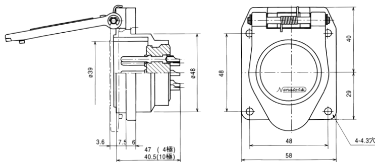
T-48*-RM
